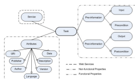
Fig. 3. Task Properties
