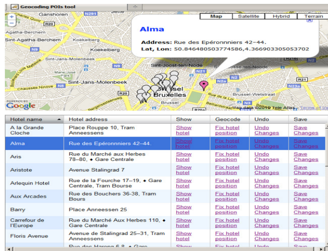
Fig. 6. Geocoding Interface
