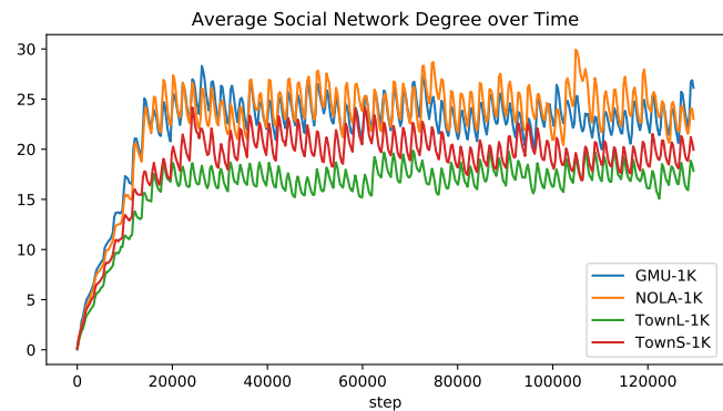
Fig. 6: Average Social Network Degree over Time (1K).
