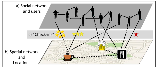
Fig. 1: LBSN Overview.
