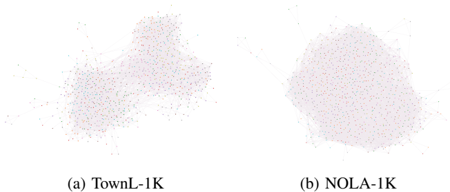
Fig. 7: Social Network.
